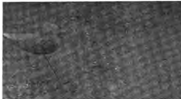
FIG. 4. Two bird-models as in Fig. 1, but out of doors against bare ground. The one on the right is obliterated, the other not.
